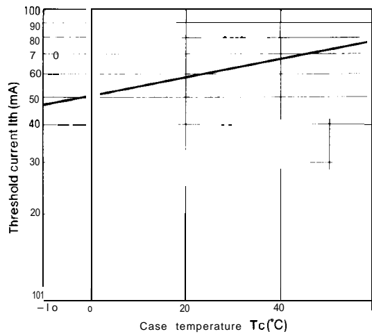
Fig. 88-3 Threshold Current vs. Temperature
