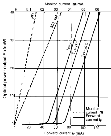
Fig. 88-3 Threshold Current vs. Temperature
