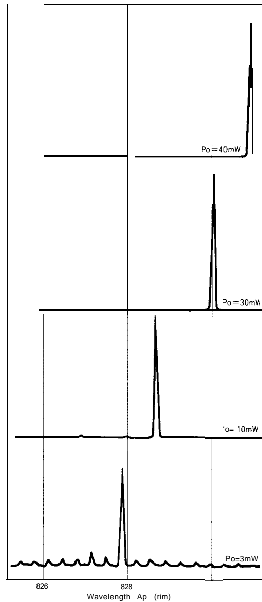
Fig. 88-5 Optical Power Output Dependence of Wavelength
